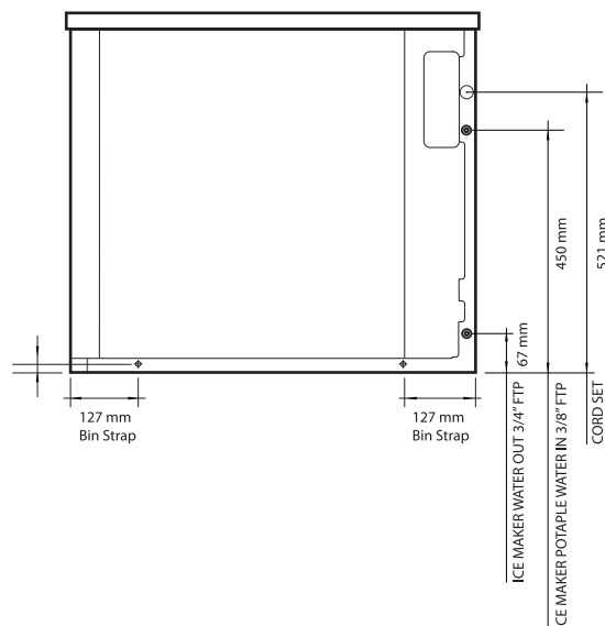
BM 805 AIR COOLED
